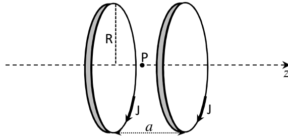
Fig.2. Helmholtz coils
